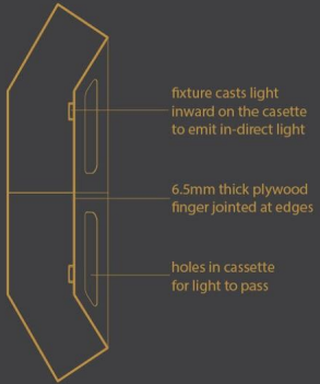
CASE STUDY LIGHTING PRECEDENT SECTION "ICD/ITKE 2011 RESEARCH PAVILION"
